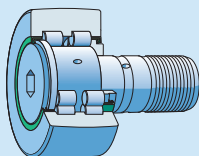
PWKR ...2RS
