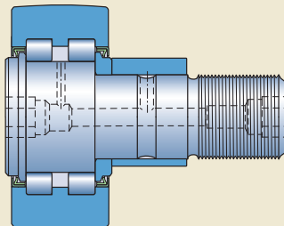
PWKRE ...2RS
