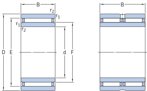
NAO
