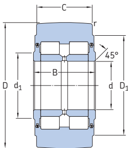
NNTR ...2ZL
